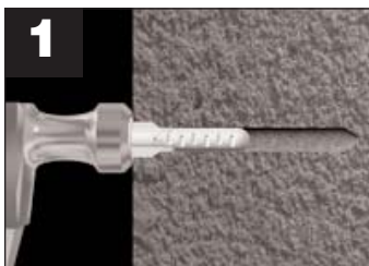
1 Drill hole same diameter as anchor. Push in anchor and tap flush.
