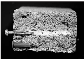
Plug anchor — NO extrusion & NO bonding
