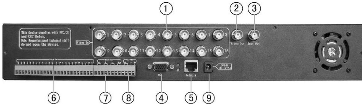
16 ch Rear Panel
